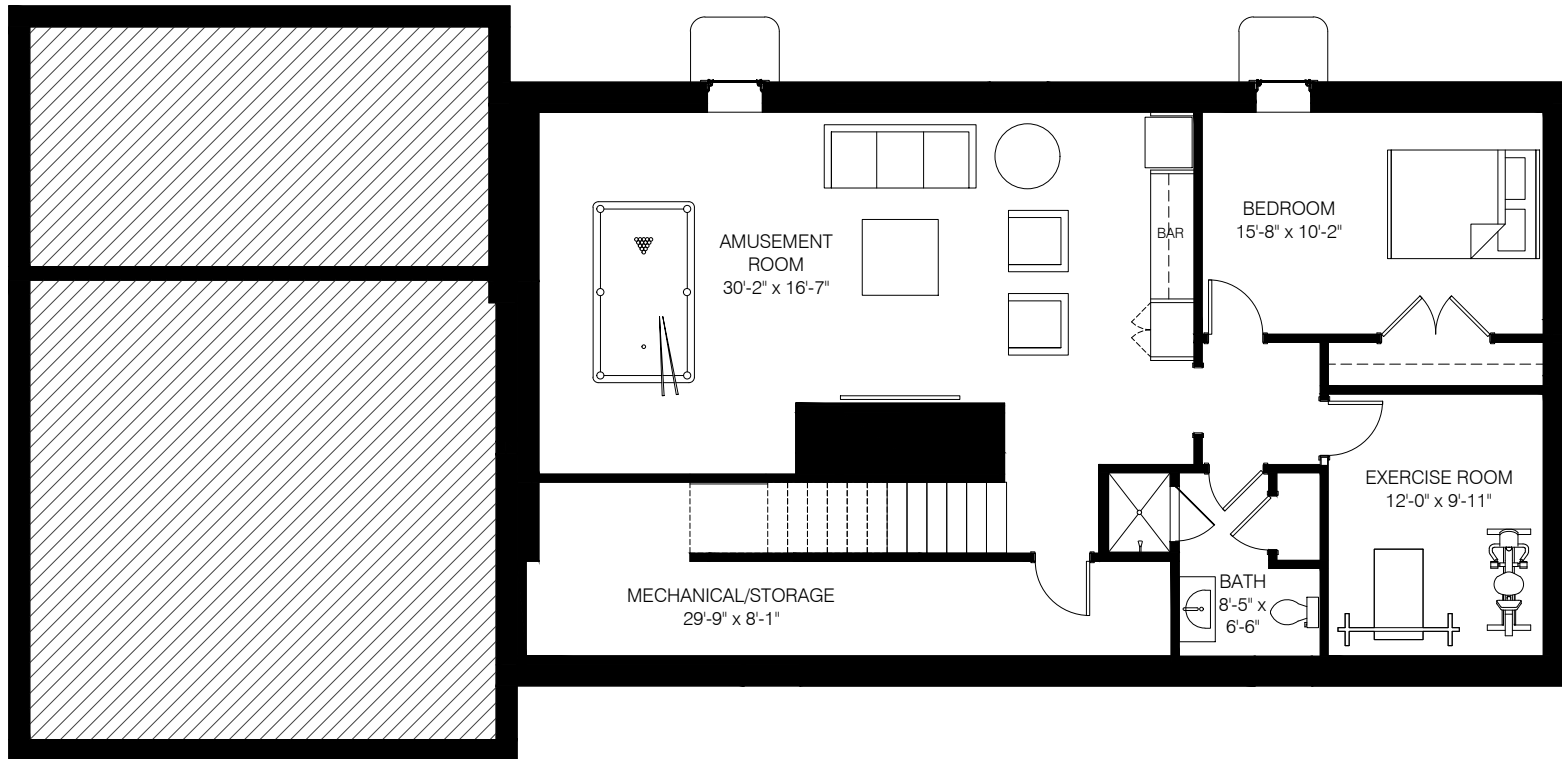
1 BASEMENT PLAN (1,119 FINISHED SQ. FT., 264 UNFINISHED SQ. FT.) A1 3/16" = 1'-0"
