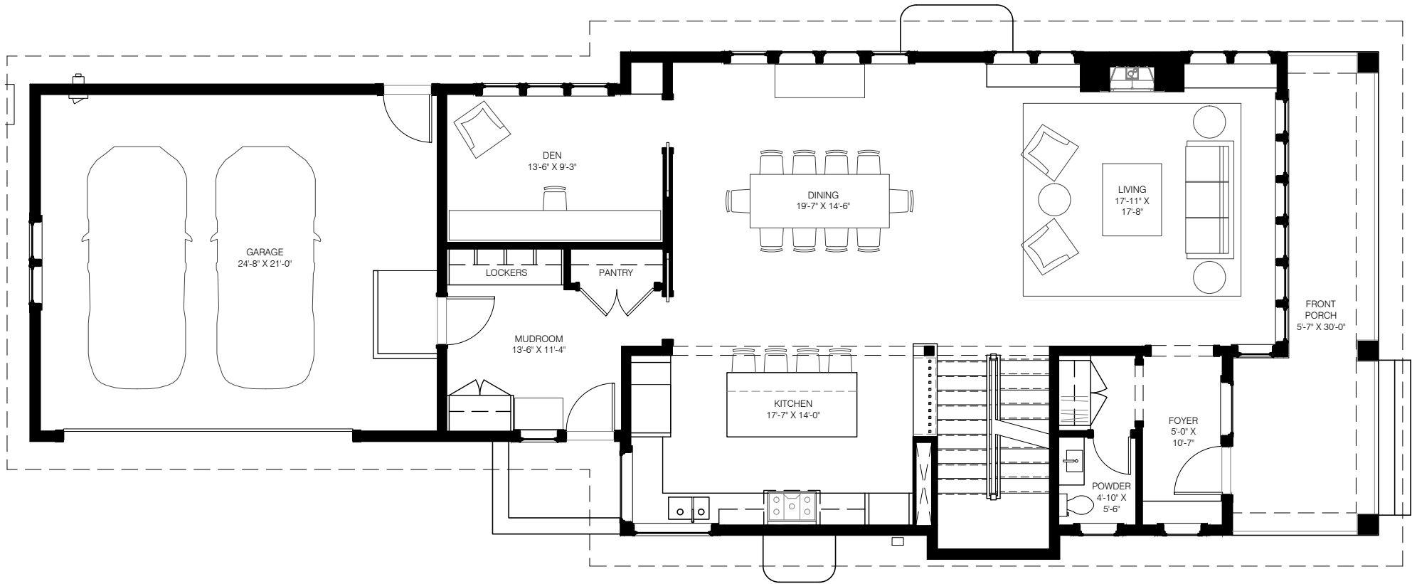
1 MAIN LEVEL PLAN (1,473 FINISHED SQ. FT.; 562 UNFINISHED SQ. FT.) A2 3/16" = 1'-0"
