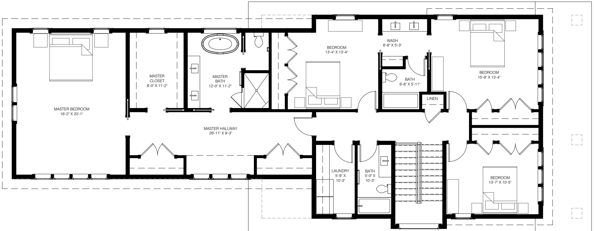
1 UPPER LEVEL PLAN (2,015 FINISHED SQ. FT.) A3 3/16" = 1'-0"
